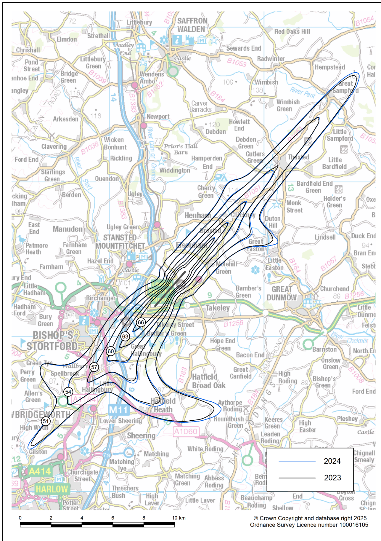
Figure B18 Stansted summer day standard modal split 2024 (72% SW / 28% NE) and 2023 (72% SW / 28% NE) L_{Aeq,16h} contours
