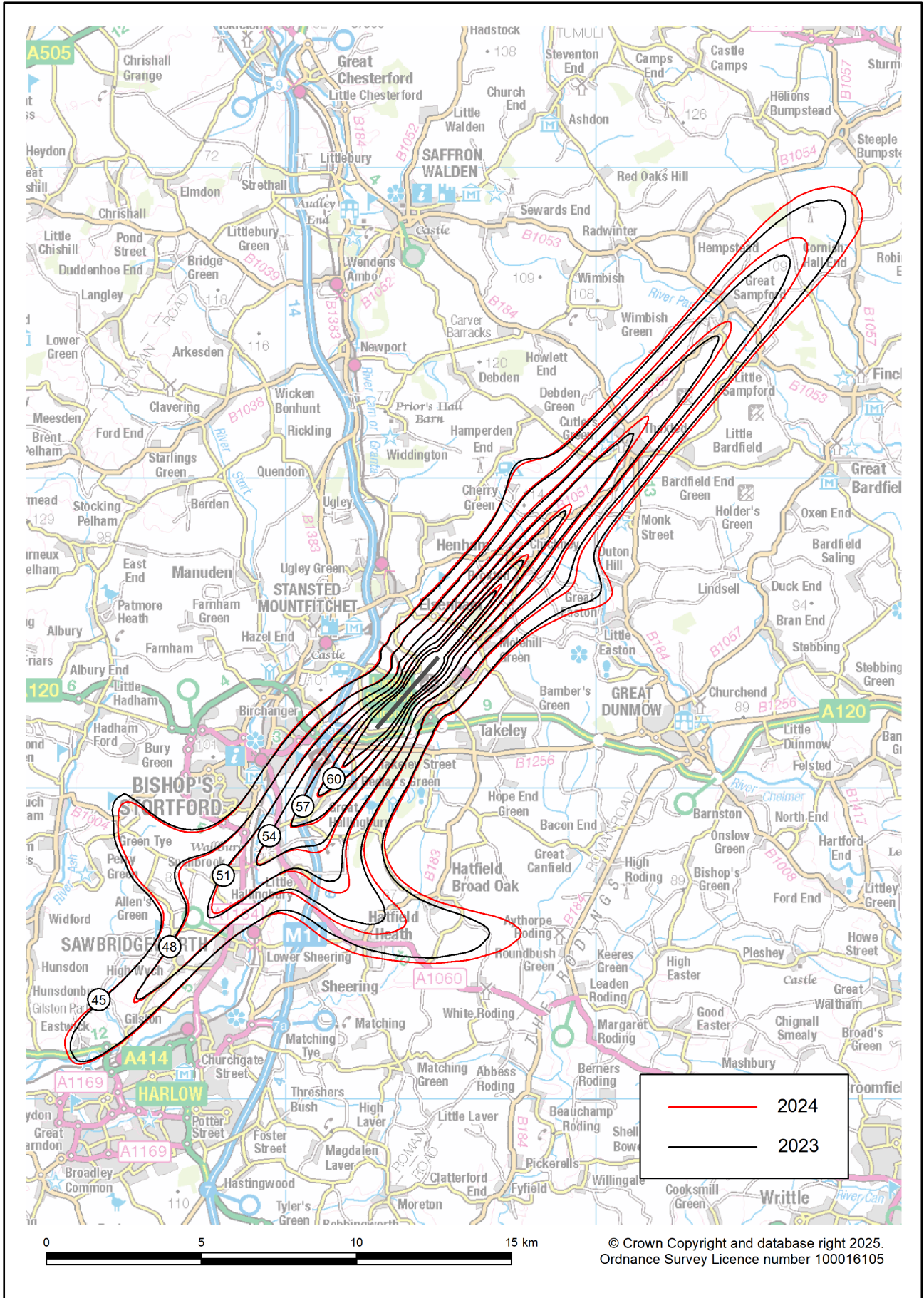
Figure B17 Stansted summer night actual modal split 2024 (78% SW / 22% NE) and 2023 (75% SW / 25% NE) L_{Aeq,8h} contours
