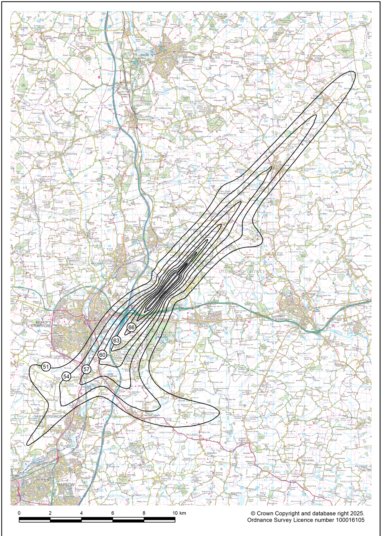
Figure B12 Stansted 2024 summer day actual modal split (76% SW / 24% NE) L_{Aeq,16h} contours
