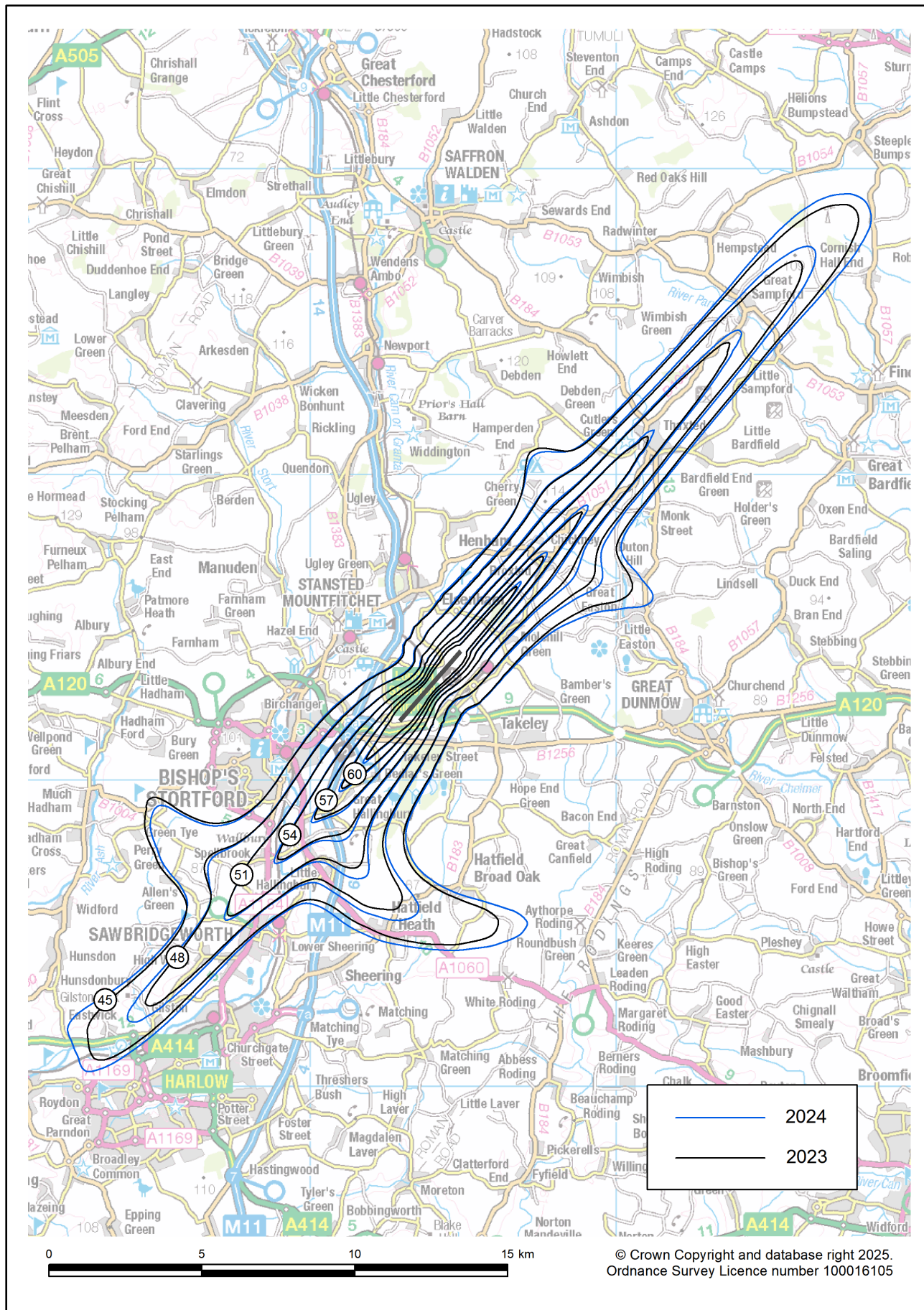
Figure B19 Stansted summer night standard modal split 2024 (71% SW / 29% NE) and 2023 (71% SW / 29% NE) L_{Aeq,8h} contours
