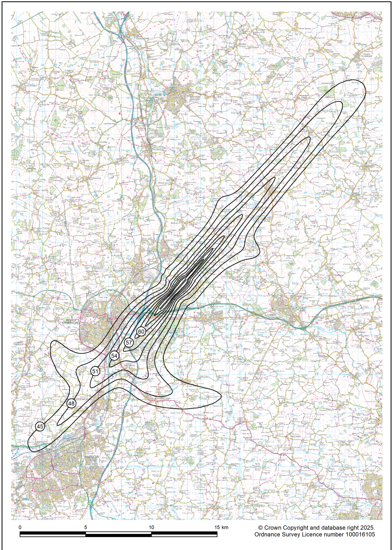
Figure B13 Stansted 2024 summer night actual modal split (78% SW / 22% NE) L_{Aeq,8h} contours
