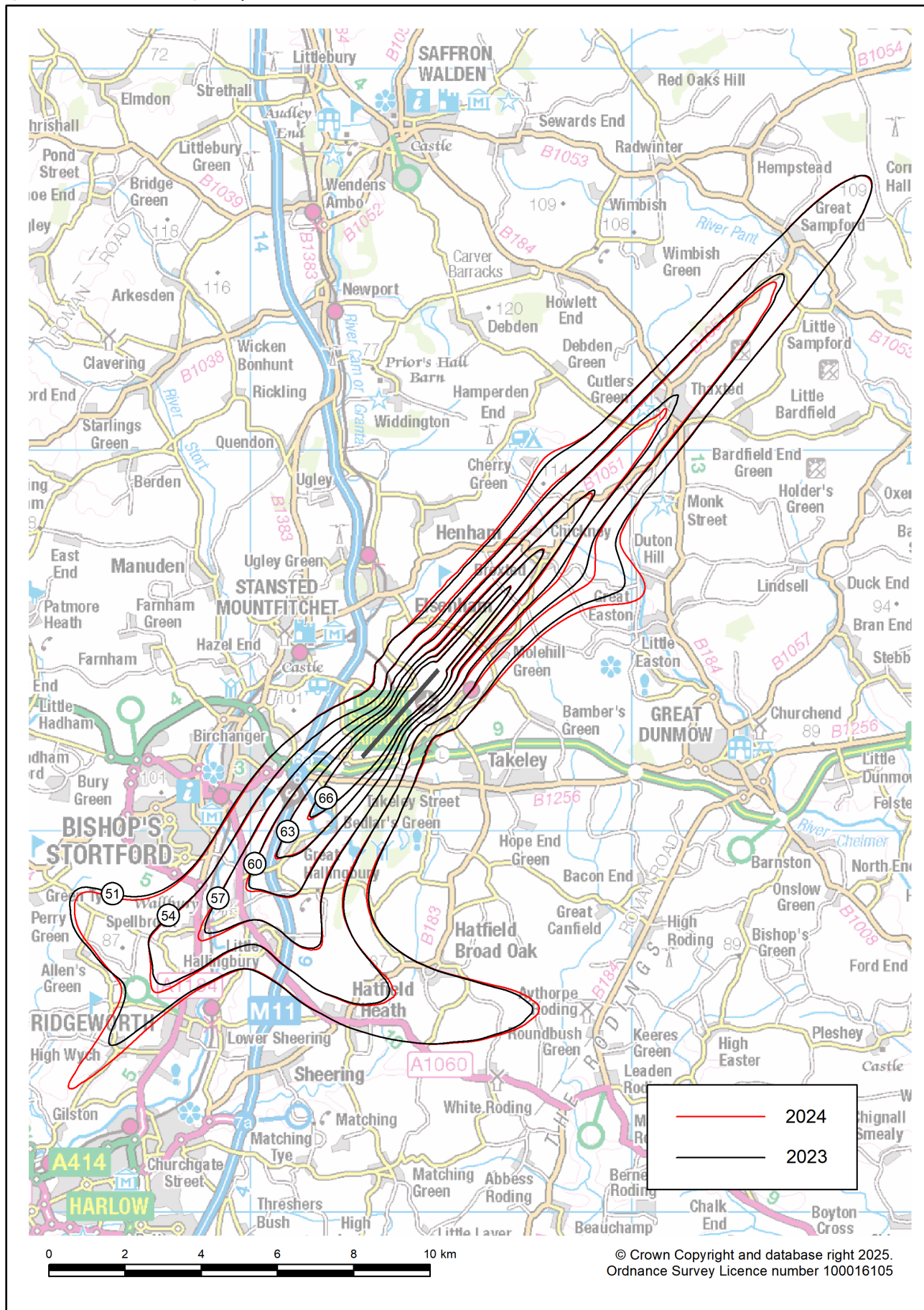
Figure B16 Stansted summer day actual modal split 2024 (76% SW / 24% NE) and 2023 (80% SW / 20% NE) L_{Aeq,16h} contours
