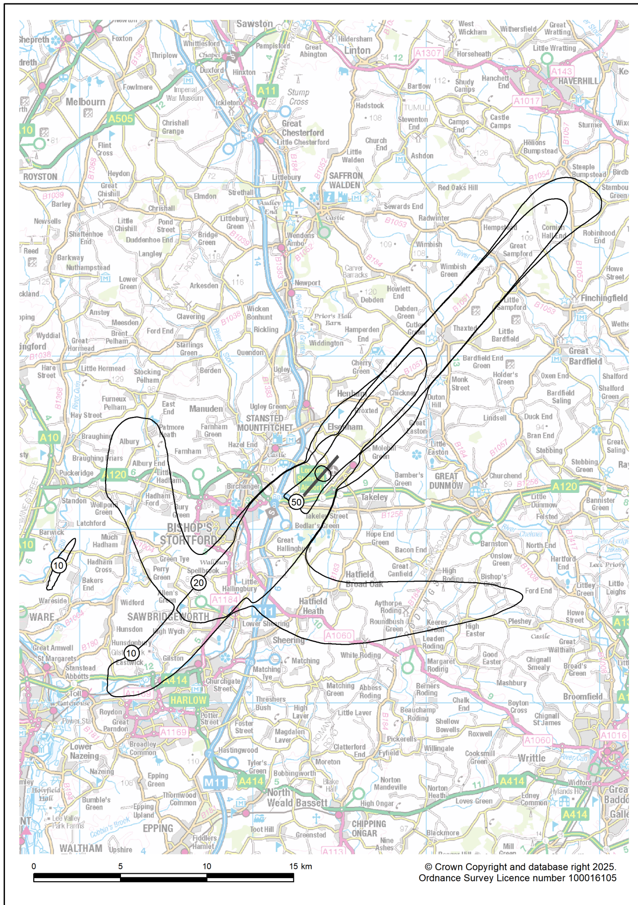
Figure B22 Stansted 2024 summer night standard modal split (71% SW / 29% NE) N60 contours
