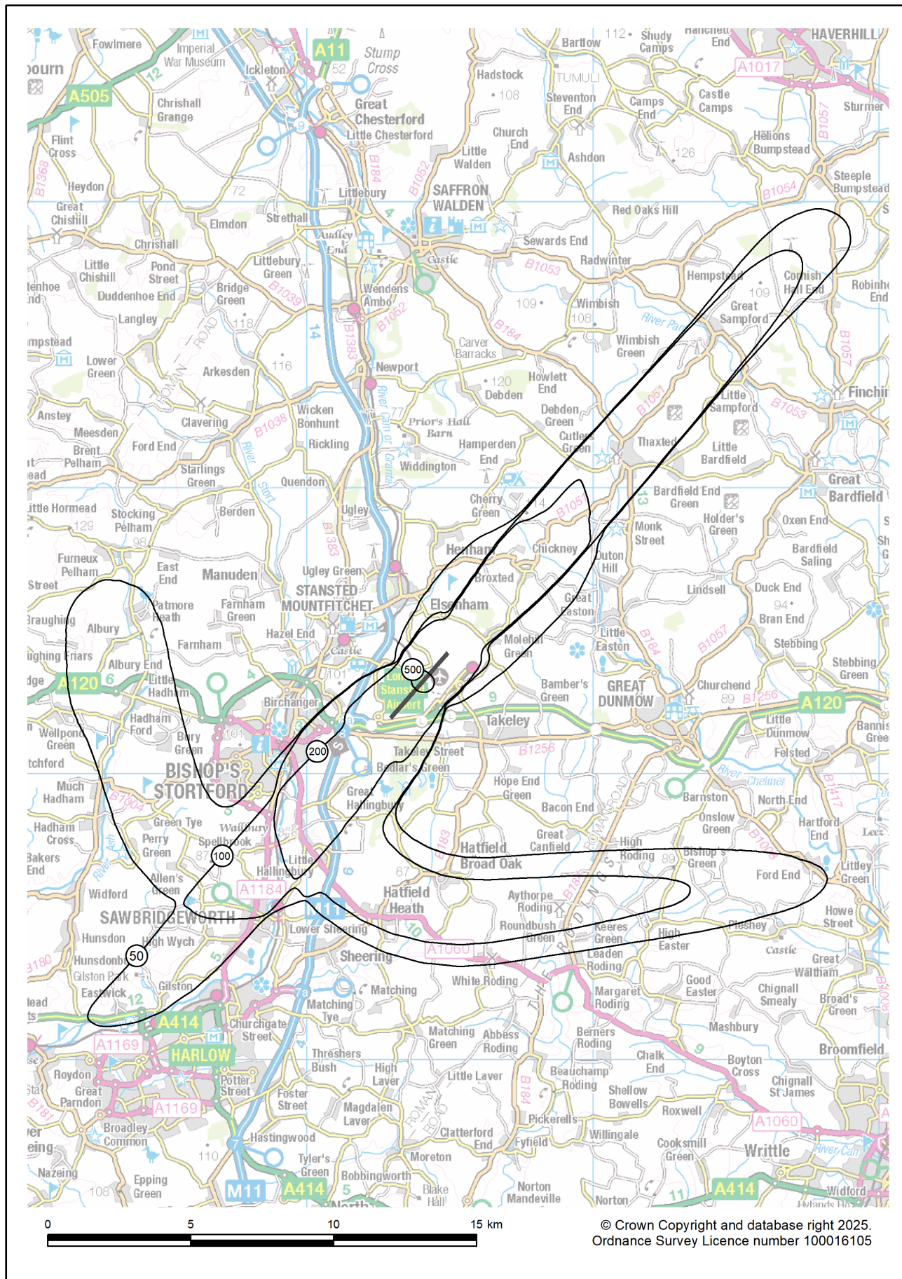
Figure B21 Stansted 2024 summer day standard modal split (72% SW / 28% NE) N60 contours
