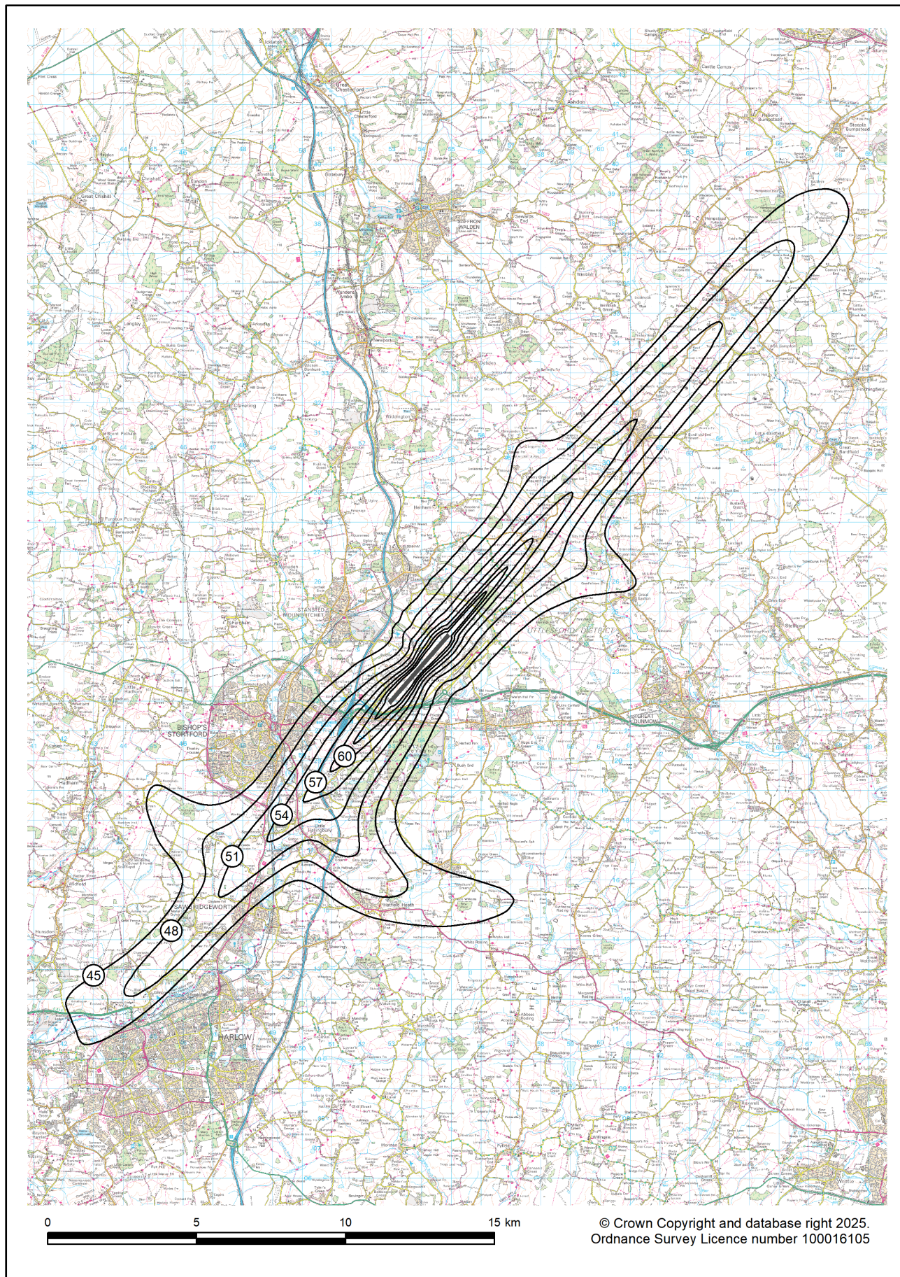
Figure B15 Stansted 2024 summer night standard modal split (71% SW / 29% NE) L_{Aeq,8h} contours
