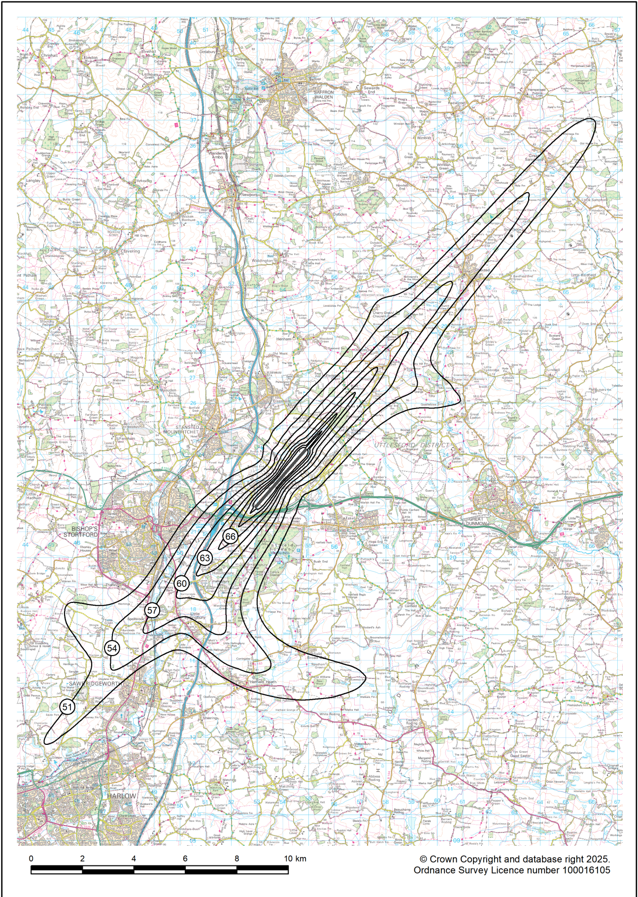
Figure B14 Stansted 2024 summer day standard modal split (72% SW / 28% NE) L_{Aeq,16h} contours
